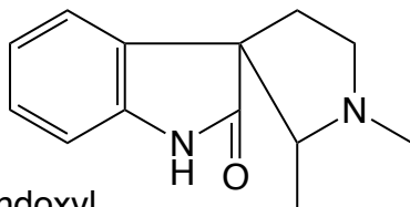
indoxyl
