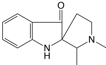
pseudoindoxyl
