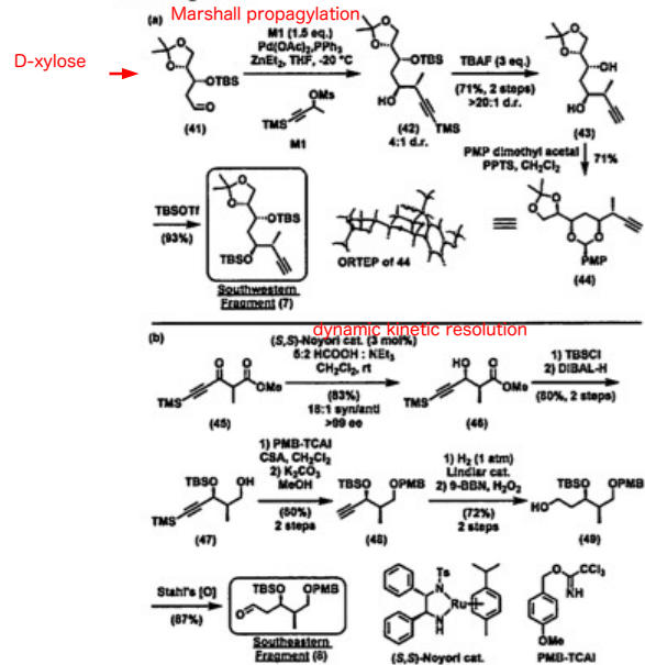
Scheme 7. Synthesis of Southwestern (7) and Southeastern (8) Fragments
