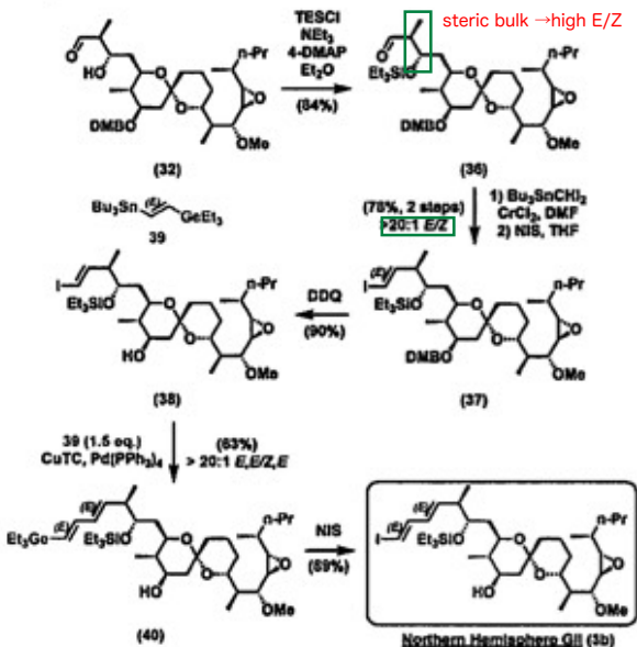
Scheme 6. Synthesis of the Second-Generation Northern Hemisphere (3b)
