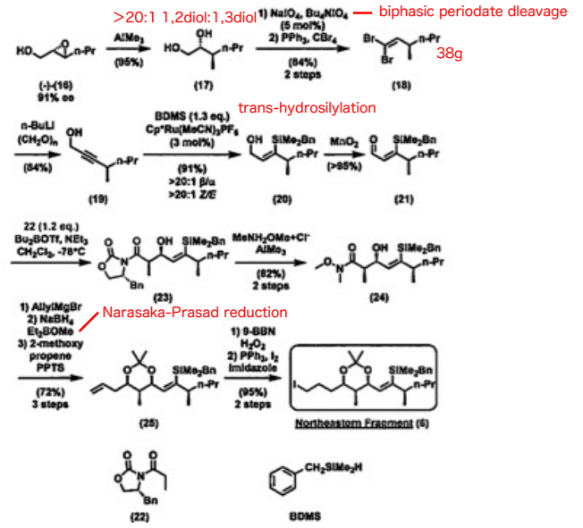
Scheme 5. Synthesis of the Northern Hemisphere (5a)
