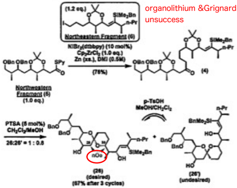
Scheme 4. Fragment Union/Spiroketalization
