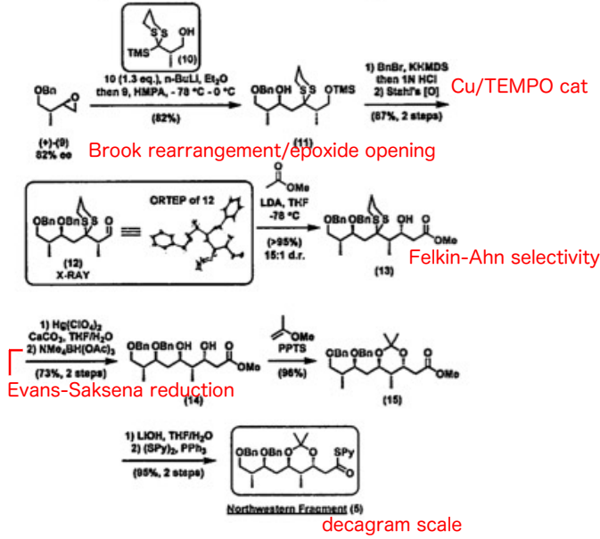
Scheme 4. Fragment Union/Spiroketalization
