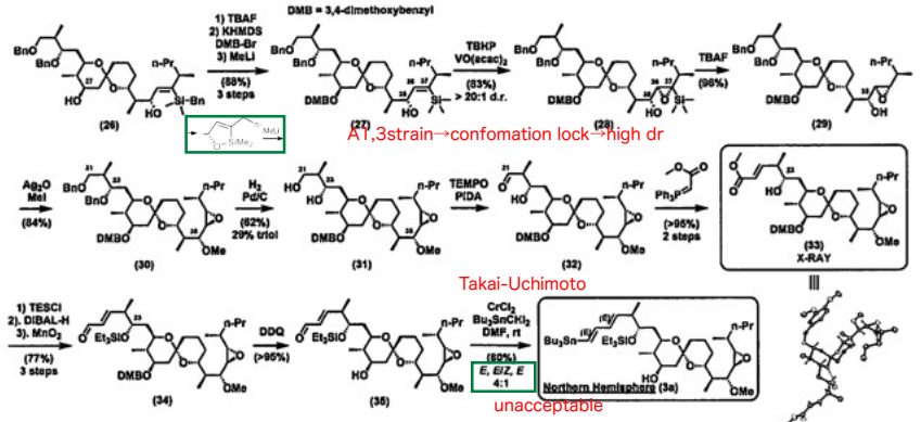
Scheme 5. Synthesis of the Northern Hemisphere (5a)
