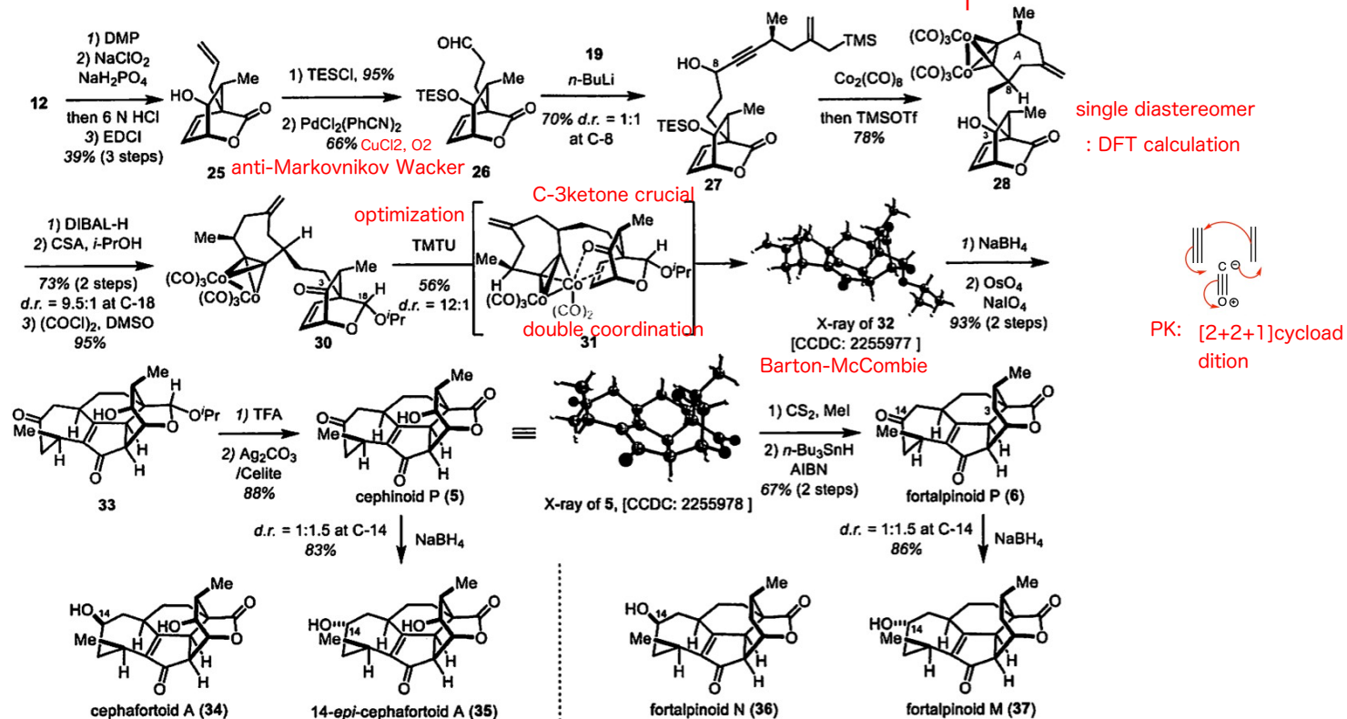
Scheme 2. Asymmetric Total Synthesis of Cephalotaxus Diterpenoids
