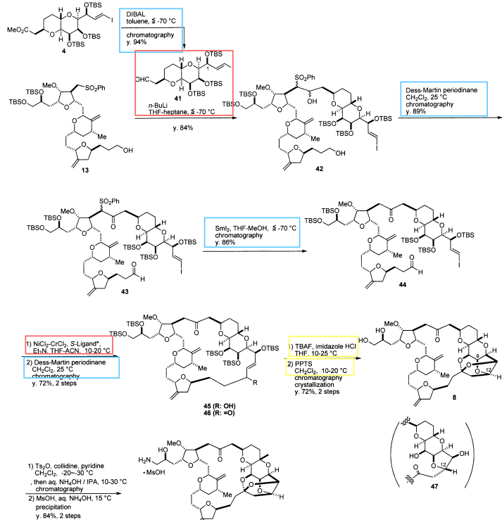
Fig. 13 Final assembly to HALAVEN™
